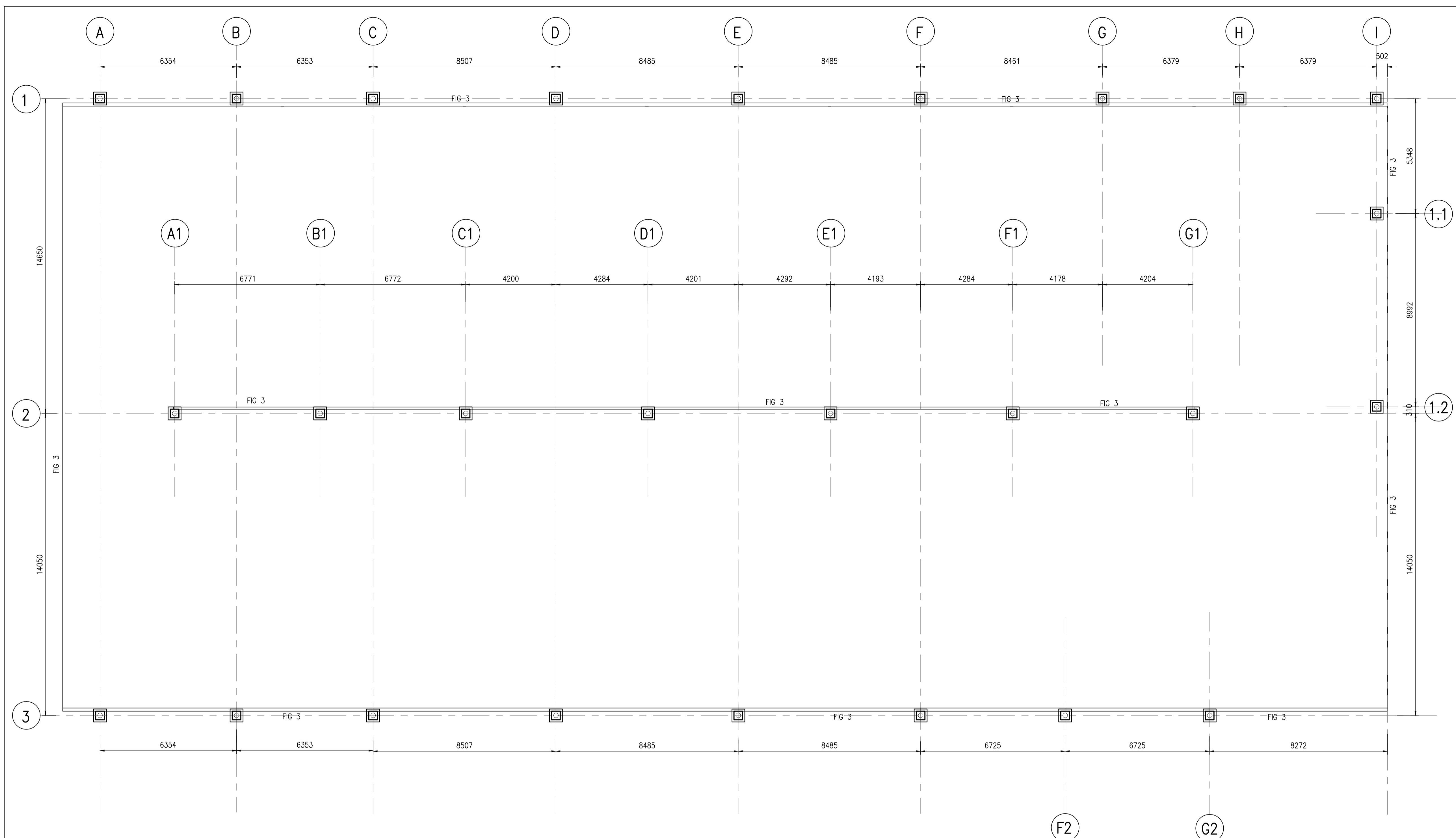
PARKING FOUNDATION LAYOUT Scale 1:100
